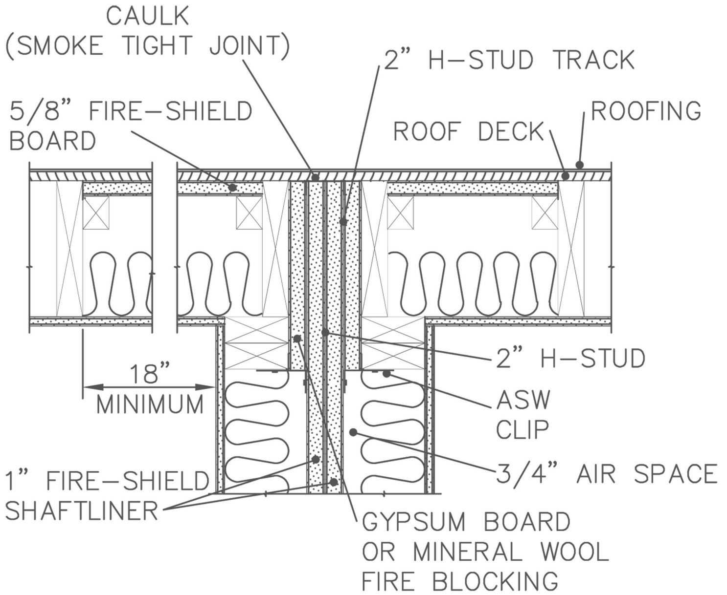
TYPICAL ROOF JUNCTION DETAIL 09265K
