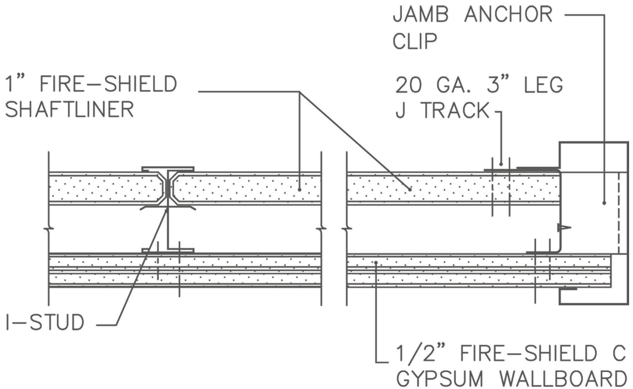
SHAFTWALL 7'-0" ELEVATOR DOOR FRAMING (SECTION A-A)
