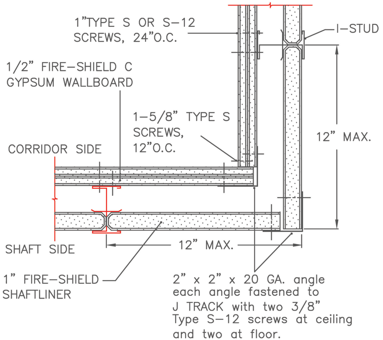
SHAFTWALL INSIDE CORNER 09260D
