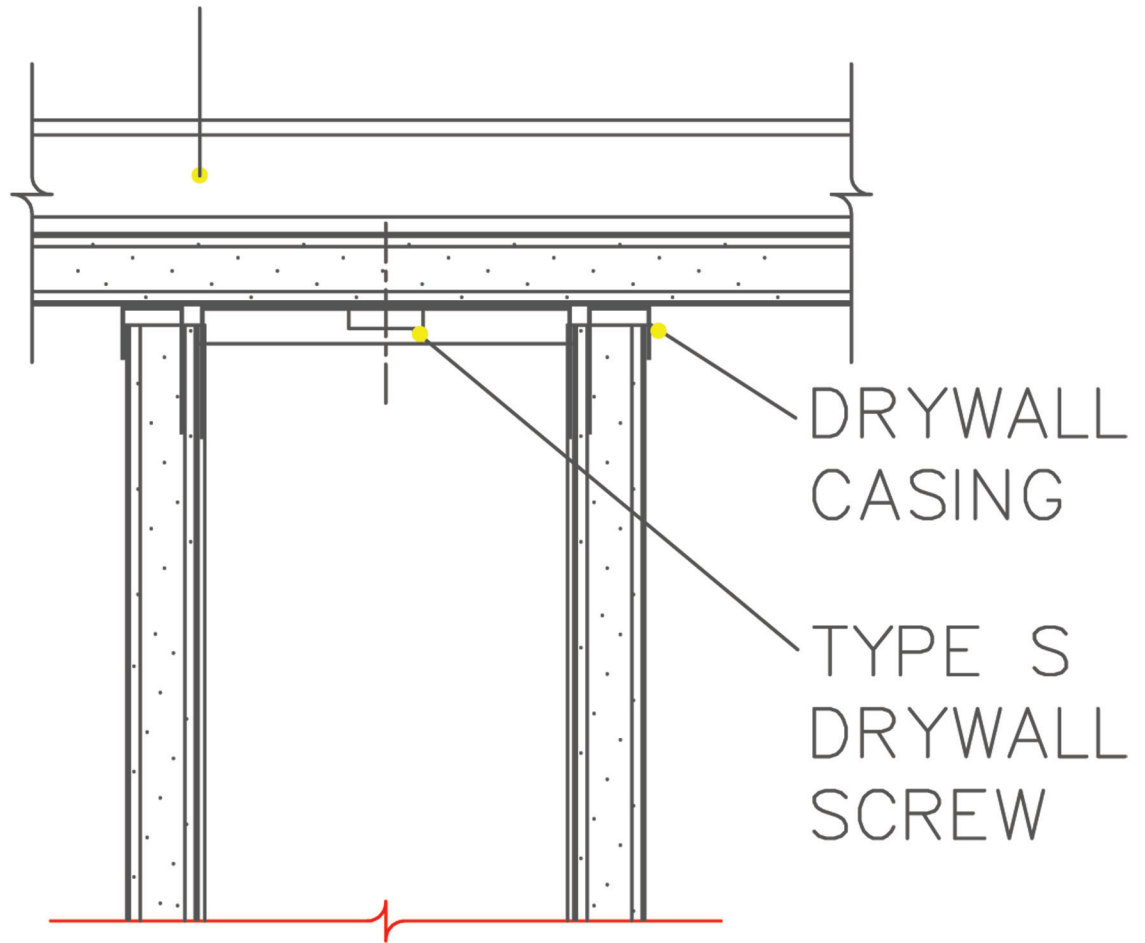
WALLBOARD PARTITION AT FURRED CEILING 09250J
