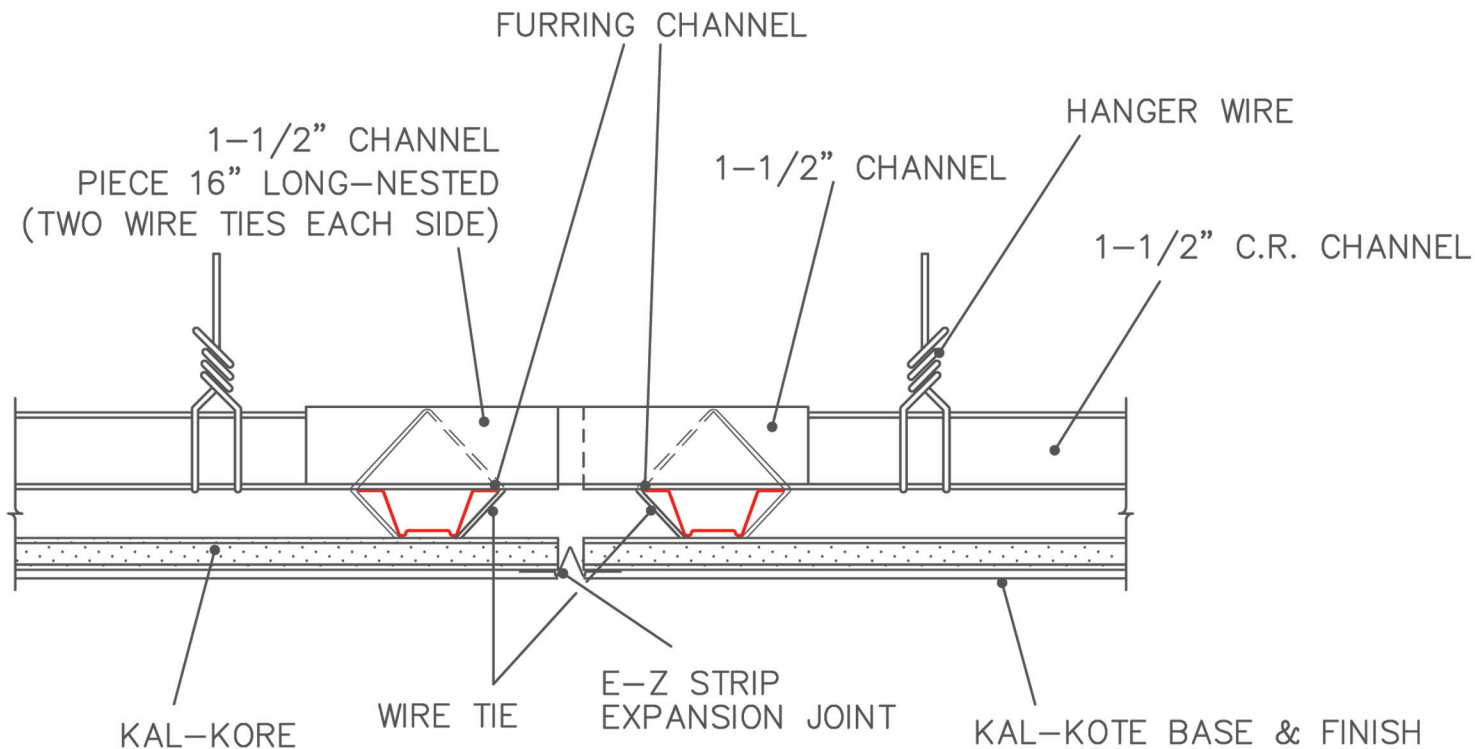
SUSPENDED WENEER PLASTER CONTROL JOINT
