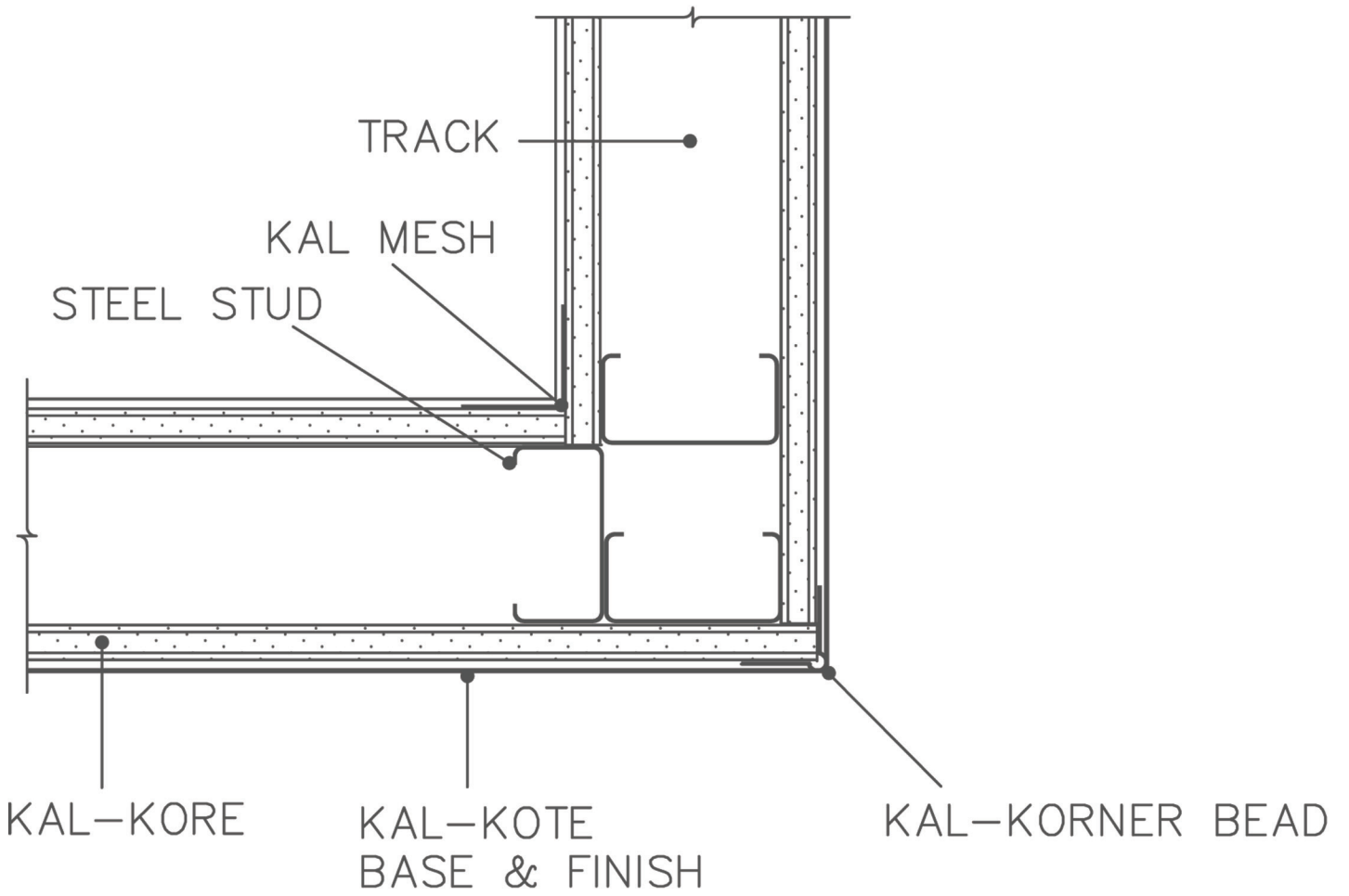
VENEER PLASTER STEEL STUD CORNER 09215B
