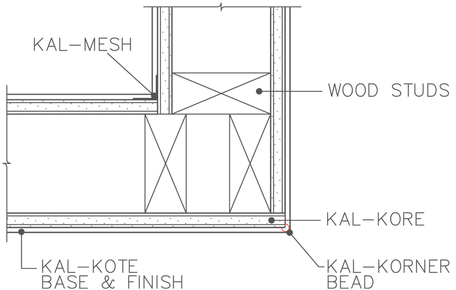
VENEER PLASTER WOOD STUD CORNER 09215A
