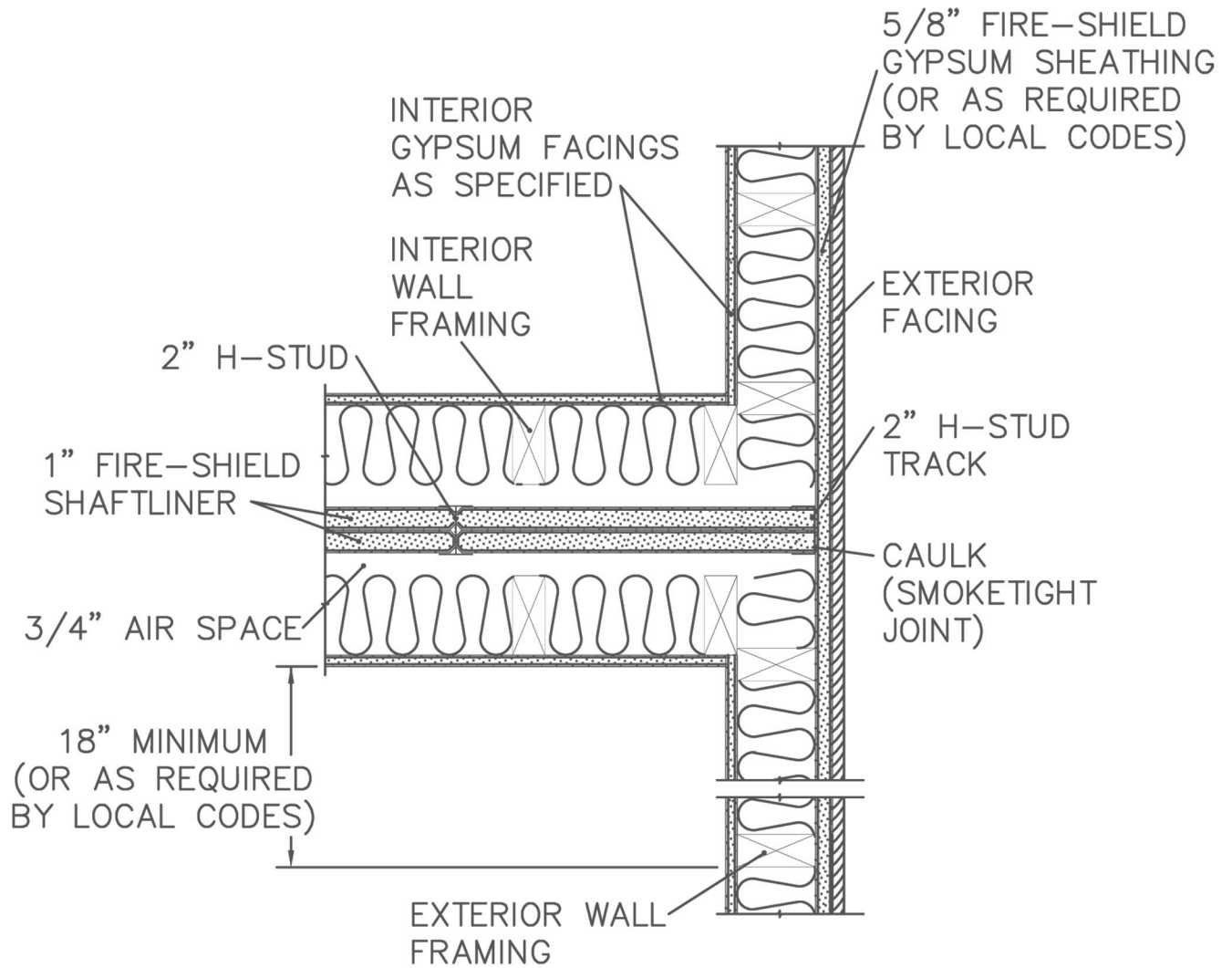
EXTERIOR WALL INTERSECTION
