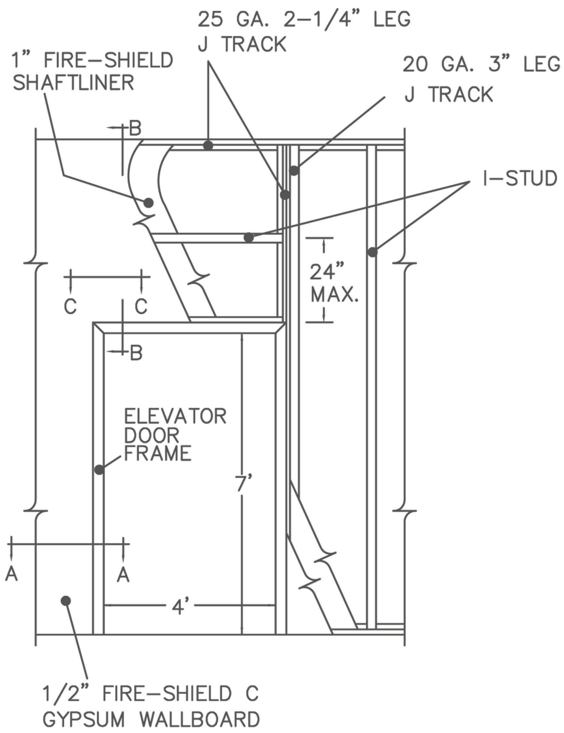
SHAFTWALL 7'-0" ELEVATOR DOOR FRAMING
