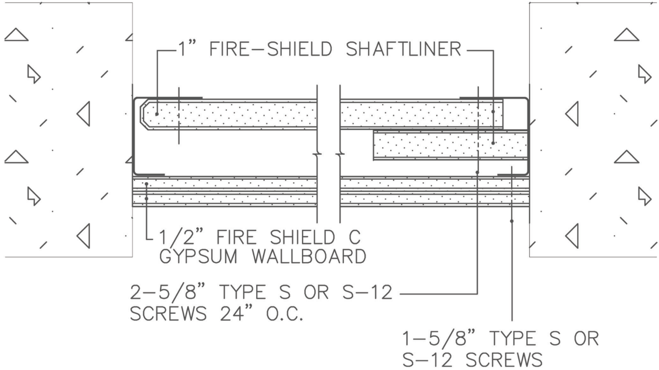
SHAFTWALL TYPICAL START AND END END OF WALL DESIGN 09260B
