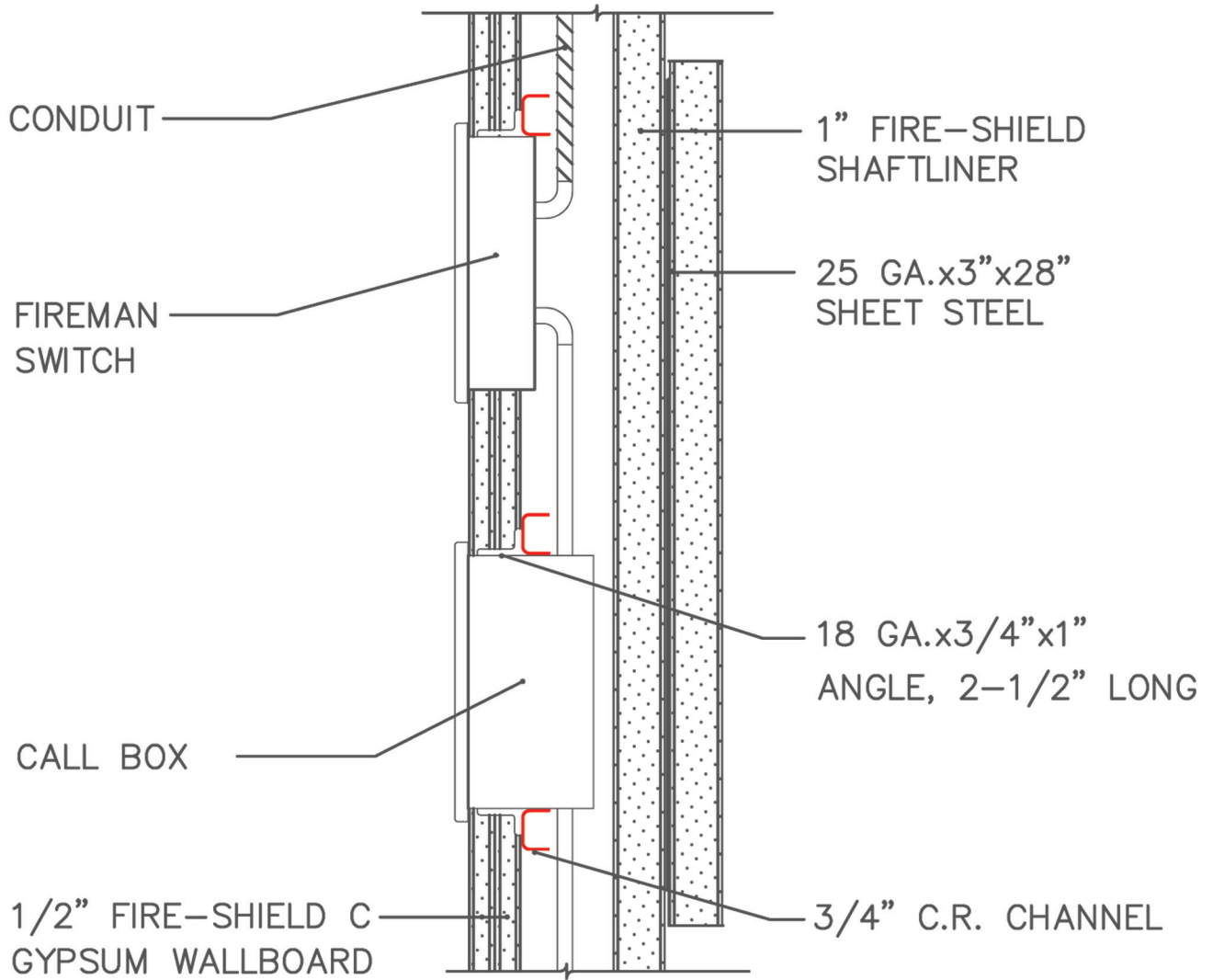
SHAFTWALL FIREMAN SWITCH AND CALL BOX
