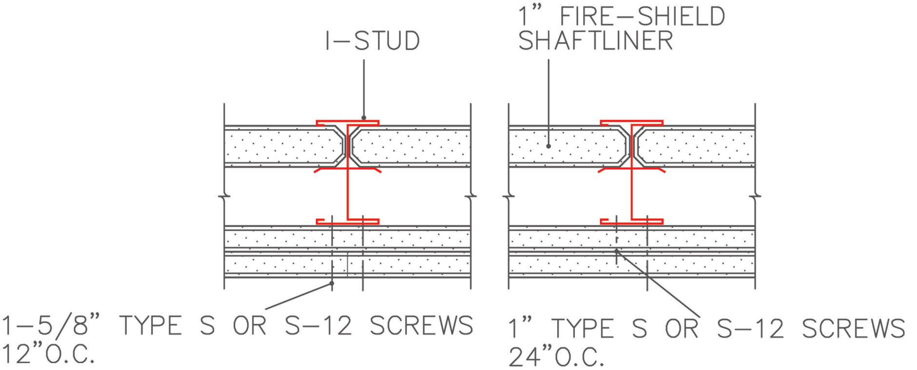
TWO HOUR FIRE RATED SHAFTWALL 09260A
